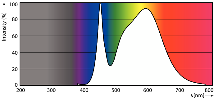
Spectral Power Distribution Colour - Sensor LEDtube 1200mm 16W 840 T8
