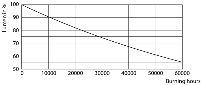
Lumen Maintenance Diagram - Sensor LEDtube 1200mm 16W 840 T8
