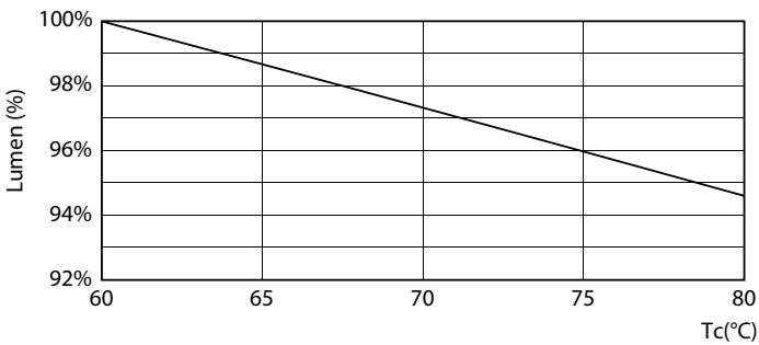
Lumen Maintenance Diagram - Ledtube DE 600mm 8W 740 T8 G13
