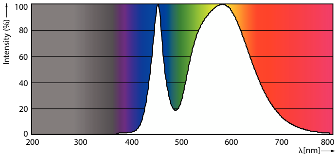
Spectral Power Distribution Colour - Ledtube DE 600mm 8W 740 T8 G13
