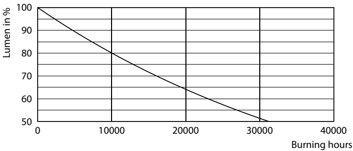
Lumen Maintenance Diagram - Ledtube DE 600mm 8W 740 T8 G13
