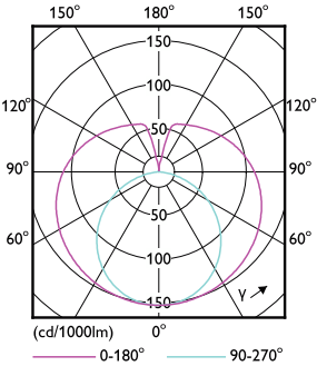
Light Distribution Diagram - Ledtube DE 600mm 8W 740 T8 G13
