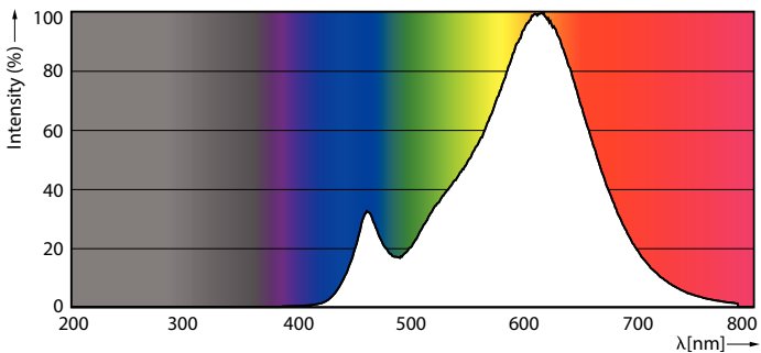
Spectral Power Distribution Colour - LEDcandle DT 6-40W E14 B38 CL CN
