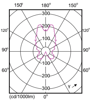
Light Distribution Diagram - LEDcandle DT 6-40W E14 B38 CL CN
