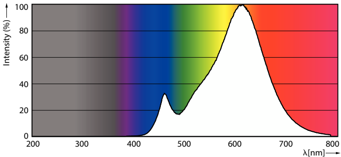
Spectral Power Distribution Colour - LEDcandle DT 4-25W E14 B38 CL CN
