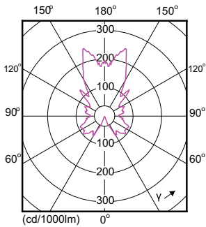
Light Distribution Diagram - LEDcandle DT 4-25W E14 B38 CL CN
