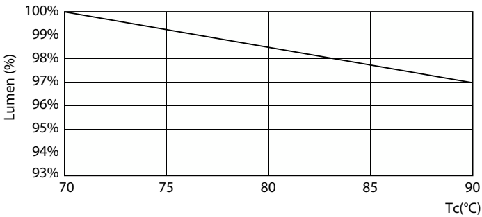
Lumen Maintenance Diagram - LED PLC 6.5W 830 2P G24d
