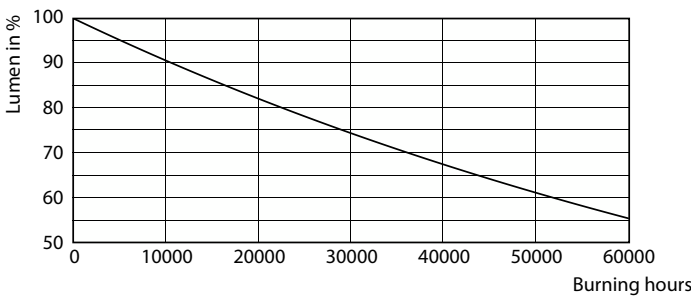
Lumen Maintenance Diagram - LED PLC 6.5W 830 2P G24d
