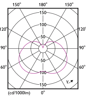
Light Distribution Diagram - LED PLC 6.5W 830 2P G24d
