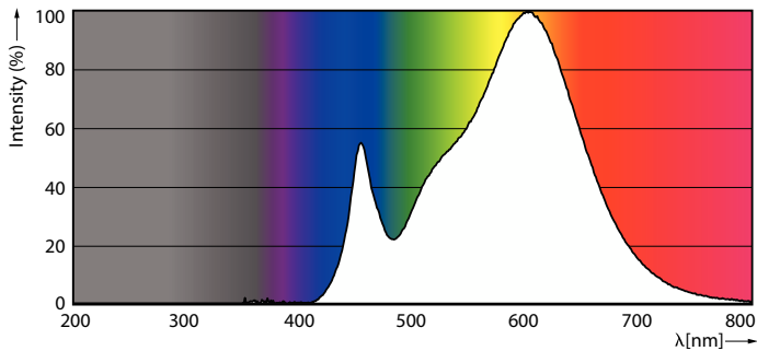
Spectral Power Distribution Colour - LED PLC 6.5W 830 2P G24d
